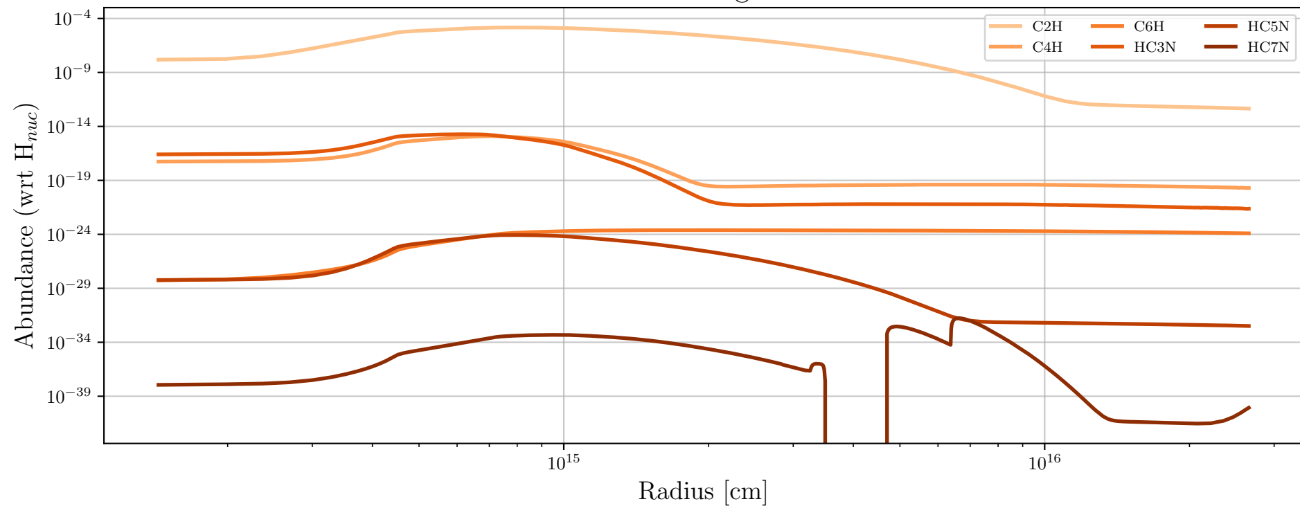
Particle 66275 - Daughter Molecules
