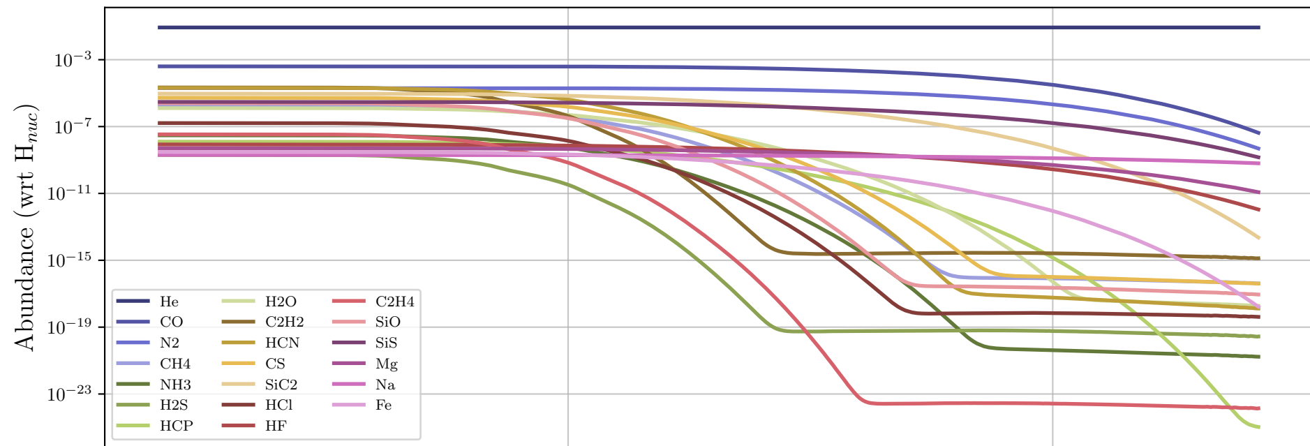
Particle 66275- Parent Molecules
